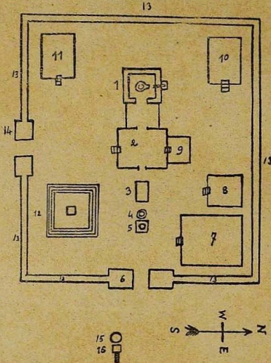
Fig. 8. Plan of a temple of Śiva
