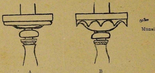
Fig. 30. Capital without Munai Capital with Munai
