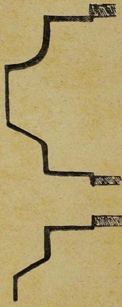
Fig. 20. Two forms of the Pallava corbel.
